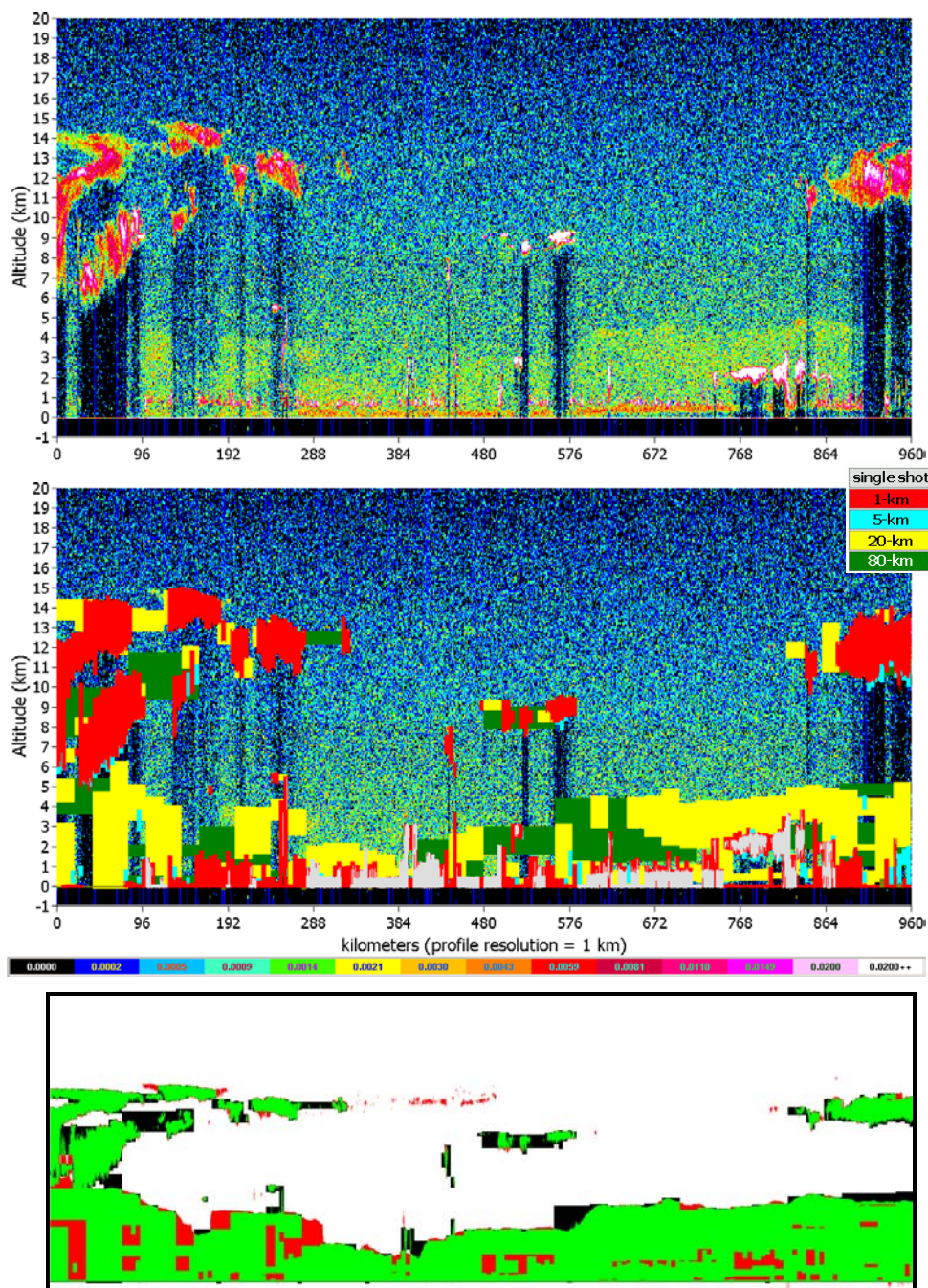
Figure 5.7: Images of simulated CALIOP data before (upper panel) and after (middle panel) being analyzed by SIBYL. The data in this scene was synthesized from retrievals performed on LITE measurements acquired during orbits 54 (clouds) and 129 (aerosols). In the middle panel, features detected at single shot resolution are rendered in pale gray; features detected at a 1-km horizontal resolution are rendered in red; 5-km features are shown in cyan; 20-km features are shown in yellow; and features detected at 80-km are shown in dark green. The lower panel presents an analysis of the feature finder results. The green regions indicate successful detection, black regions represent false positives, and red regions show missed features.
