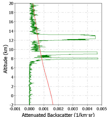
Figure 7.3: LITE profile from orbit 54 at 7.349° S, 52.846° W
