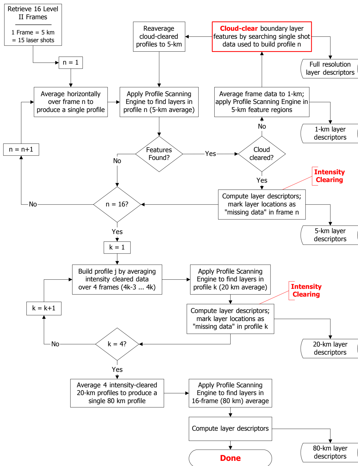
Figure 4.17: SIBYL Internals
