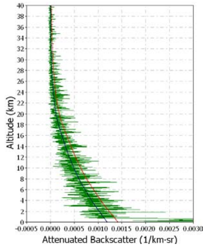
Figure 3.4: LITE Data with Threshold = \beta_{air}(z) + 3 \cdot RBV(z)
