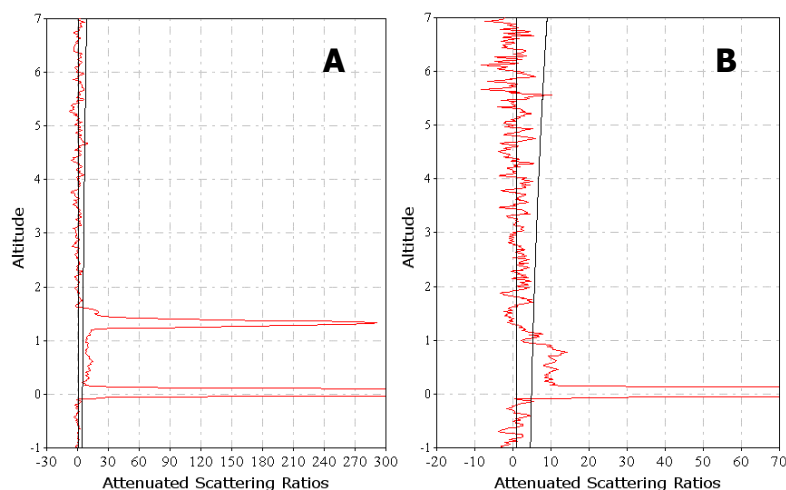
Figure 4.11: LITE 1064 nm attenuated scattering ratios for two consecutive 5-km segments; segment A shows fair weather cumulus embedded in aerosol, while segment B contains a single cloud-free aerosol layer
