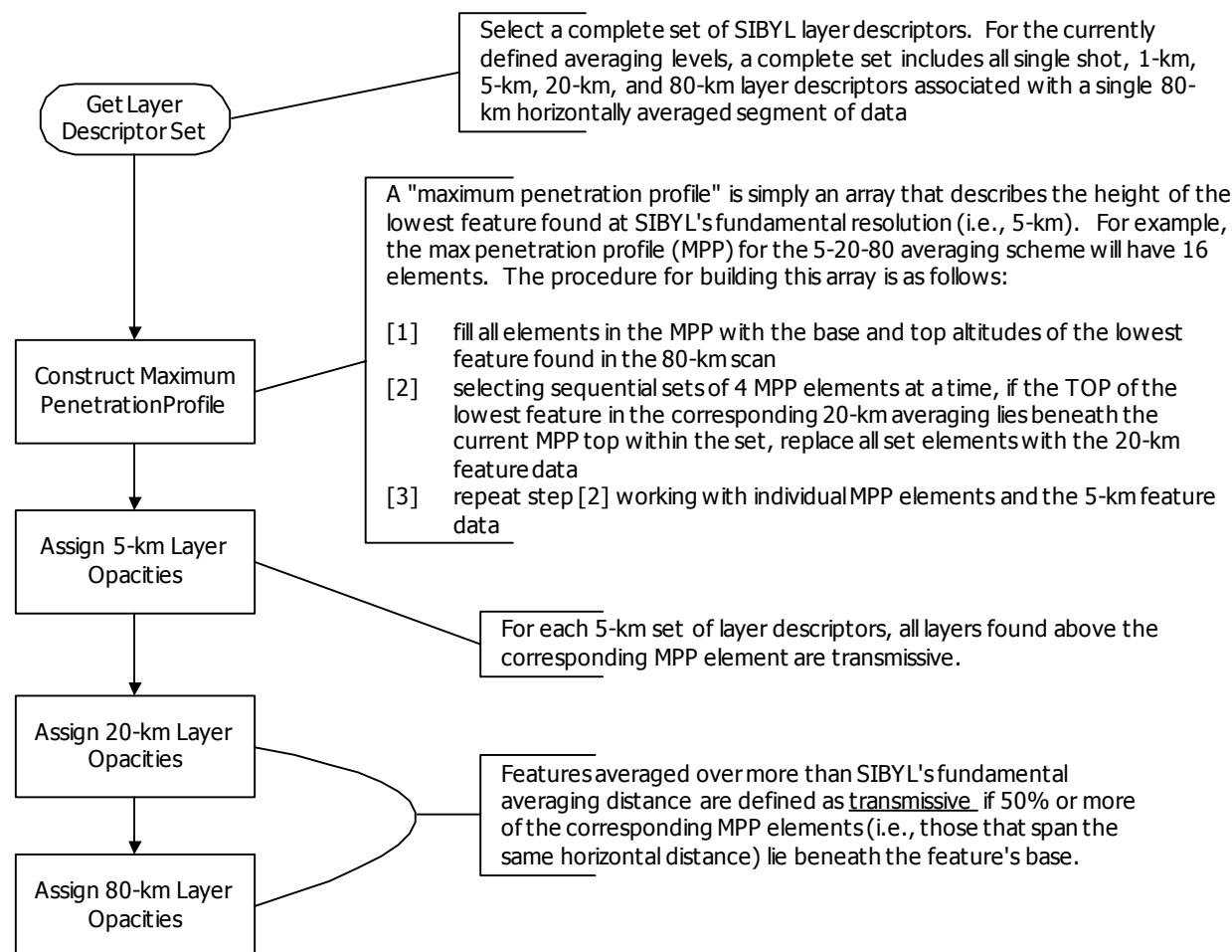
Figure 7.4: Layer opacity procedure
