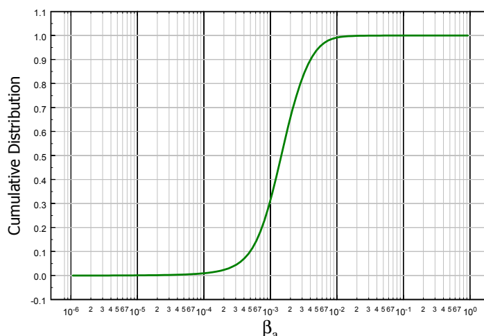
Figure 4.15: Distribution of aerosol backscatter coefficients retrieved from LITE data using S^*=25
