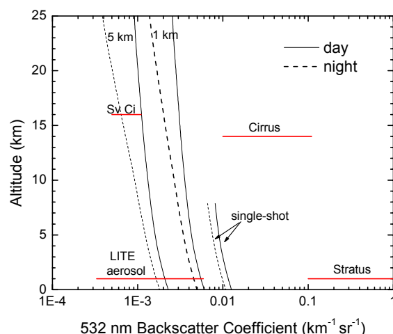
Figure 2.3: Detection sensitivity of CALIOP 532 nm channel on single shot profiles and profiles horizontally averaged to 1 km and 5 km
