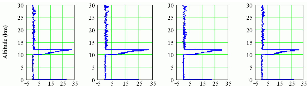
Figure 4.3: 5-km Attenuated Scattering Ratio Profiles
