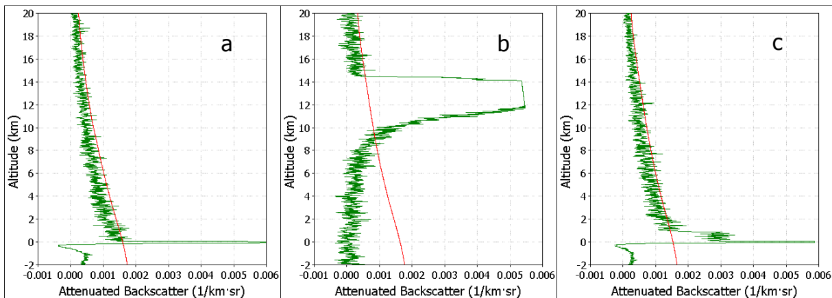
Figure 7.1: The three classes of surface returns: (a) a “pure” surface return, (b) no surface return detected, and (c) surface return in contact with an atmospheric feature. All profiles shown were acquired during LITE orbit 148, between 45° N and 35° N. The smooth red line in each image represents the initial profile scanner threshold that would be used in the search routine.
