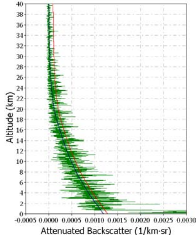
Figure 3.3: LITE Data with Threshold = \beta_{\text{air}}(z) + 3 \cdot \text{MBV}
