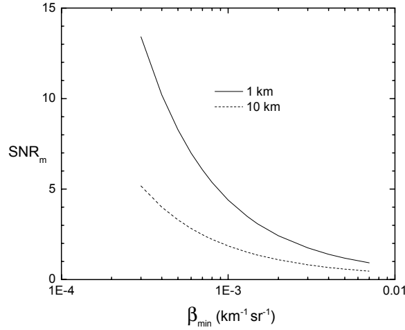
Figure 2.2: SNR required to detect layer with 532 nm backscatter coefficient of \beta_{532} \text{ (km}^{-1} \text{ sr}^{-1}\text{)} at two altitudes, 1 km and 10 km, parameterized in terms of the SNR in clear air outside the layer, \text{SNR}_m . This example for night conditions with 90% detection probability and 10% false alarm rate ( x_d = x_{fa} = 1.28 ).
