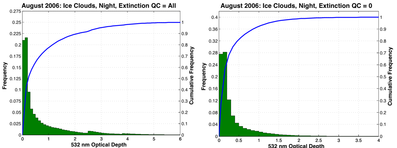
Figure 2: CALIPSO cirrus cloud optical depths (v3.01 - August 2006, nighttime only)
