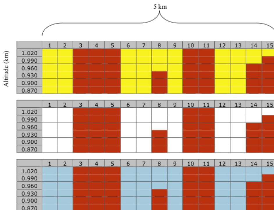
Figure 4: Cloud clearing scenarios for strongly scattering clouds detected at single shot resolution. Red indicates clouds detected at 1/3 km resolution, blue indicates clouds found at 1 km or coarser resolution, yellow indicates an aerosol layer found at 5 km resolution, and white indicates clear air. Scenarios: Clouds embedded in aerosol (upper panel), clouds embedded in clear air (middle panel), and dense clouds embedded in within a weakly scattering cloud layer (lower panel). Each row extends 5 km horizontally and 30 m vertically. Each column extends 1/3 km horizontally.
