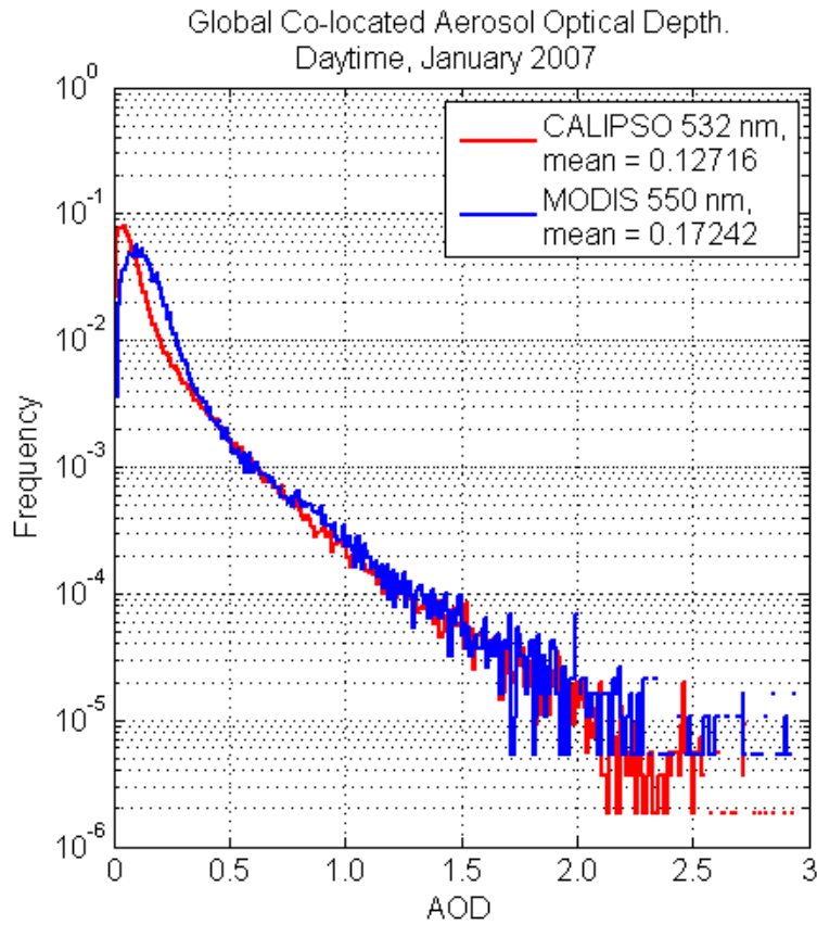
Figure 1: Comparison of CALIPSO aerosol optical depths to those derived from MODIS (Preliminary - January 2007, daytime data, final lidar ratio = initial lidar ratio only )
