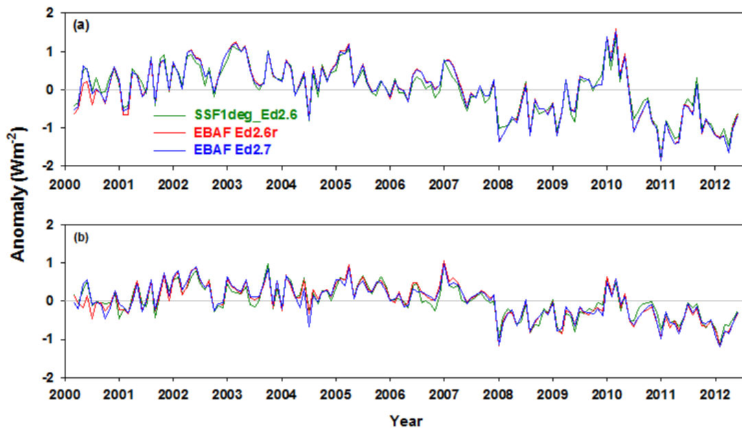
Figure 5-9. Monthly clear-sky LW TOA flux anomalies for (a) 30^\circ S-30^\circ N and (b) global.
