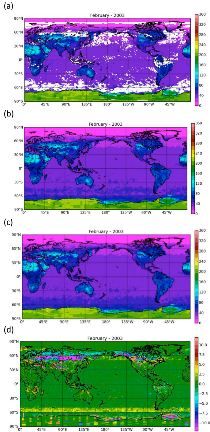
Figure 5-5. February 2003 monthly mean clear-sky SW TOA flux for (a) CERES Terra SSF1deg-lite_Ed2.6, (b) EBAF Ed2.6r, (c) EBAF Ed2.7, and (d) EBAF Ed2.7 minus EBAF Ed2.6r. Units in W m^{-2} .
