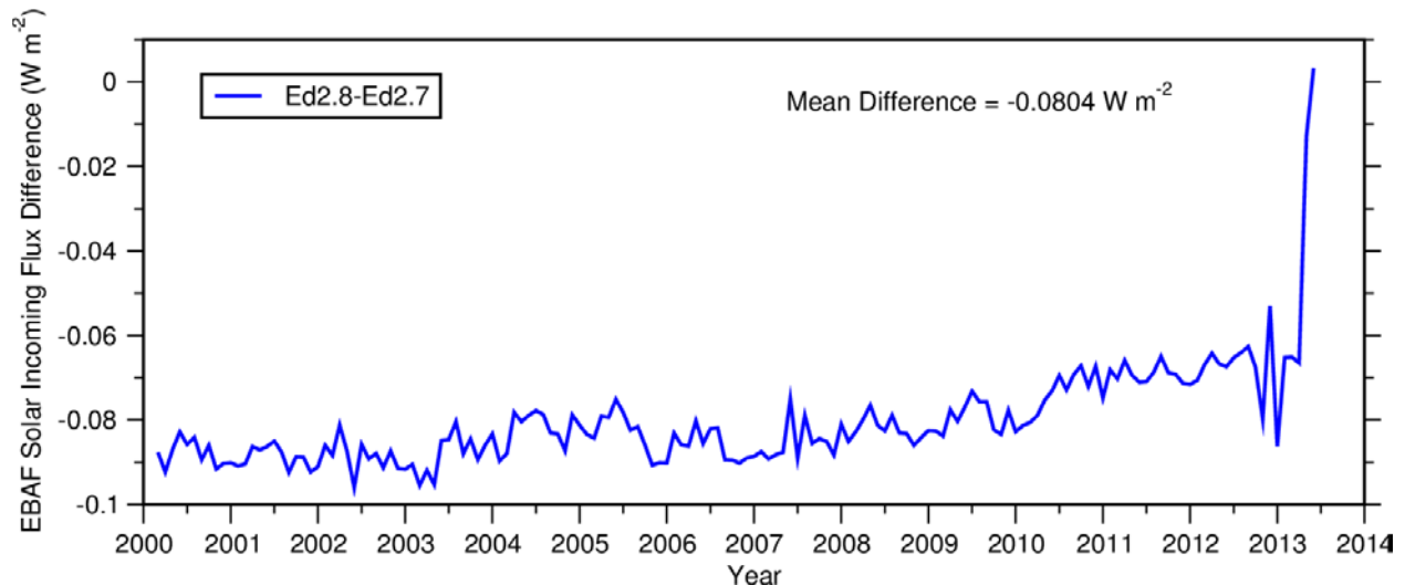
Figure 5-2. Difference in global monthly mean solar incoming flux between EBAF Ed2.8 and EBAF Ed2.7 from March 2000 through June 2013 ( \text{W m}^{-2} ).
