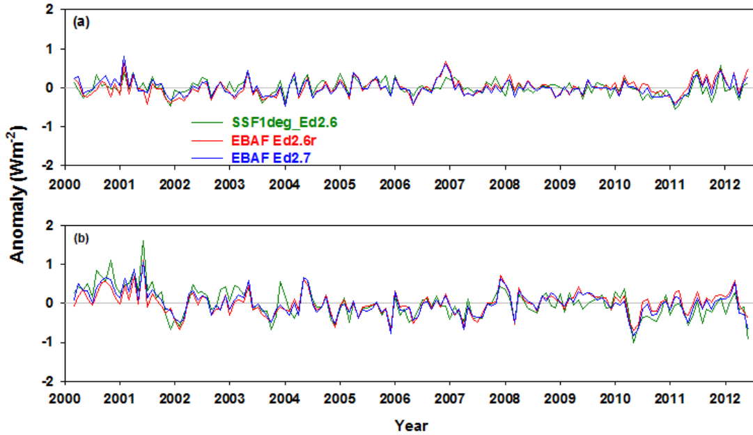
Figure 5-8. Monthly clear-sky SW TOA flux anomalies for (a) 30^\circ S-30^\circ N and (b) global.
