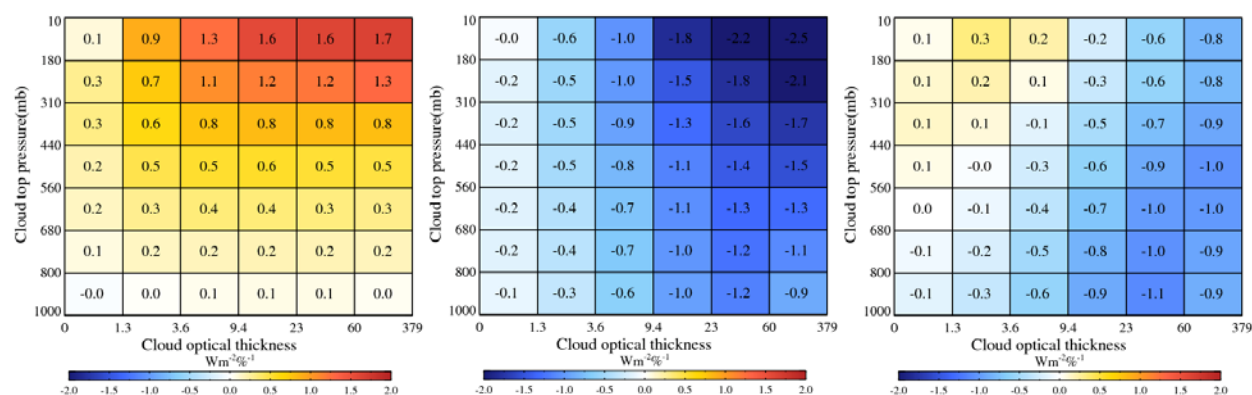
Figure 5-8. The 2010 FluxByCldTyp LW (left panel), SW (middle panel), and Net (right panel) global mean TOA flux radiative kernel in \text{W m}^{-2} \%^{-1} . Compare to Figure 1 in Zelinka et al. (2012).
