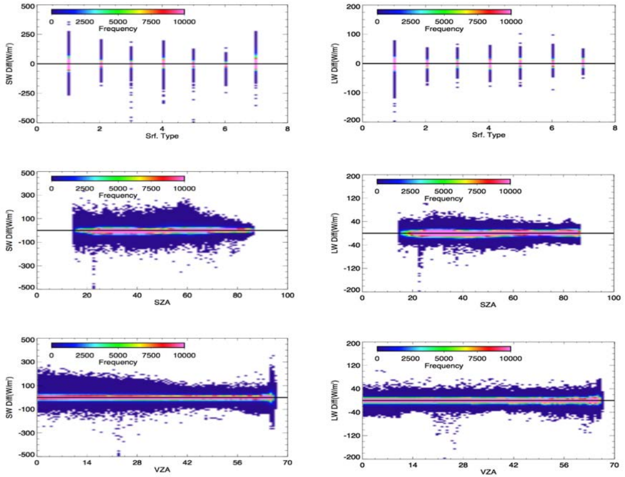
Figure 5-3. The FluxByCldTyp narrowband to broadband computed minus observed (left panels) SW and (right panel) LW non-homogeneous Terra and Aqua footprint flux ( \text{W m}^{-2} ) frequency plots during January 1-10, 2010 as a function of surface type (1=ocean, 2=forest, 3=savanna, 4=grass/croplands, 5=dark deserts, 6=bright deserts, 7=snow/ice), solar zenith angle (SZA in degrees) and view zenith angle in degrees.
