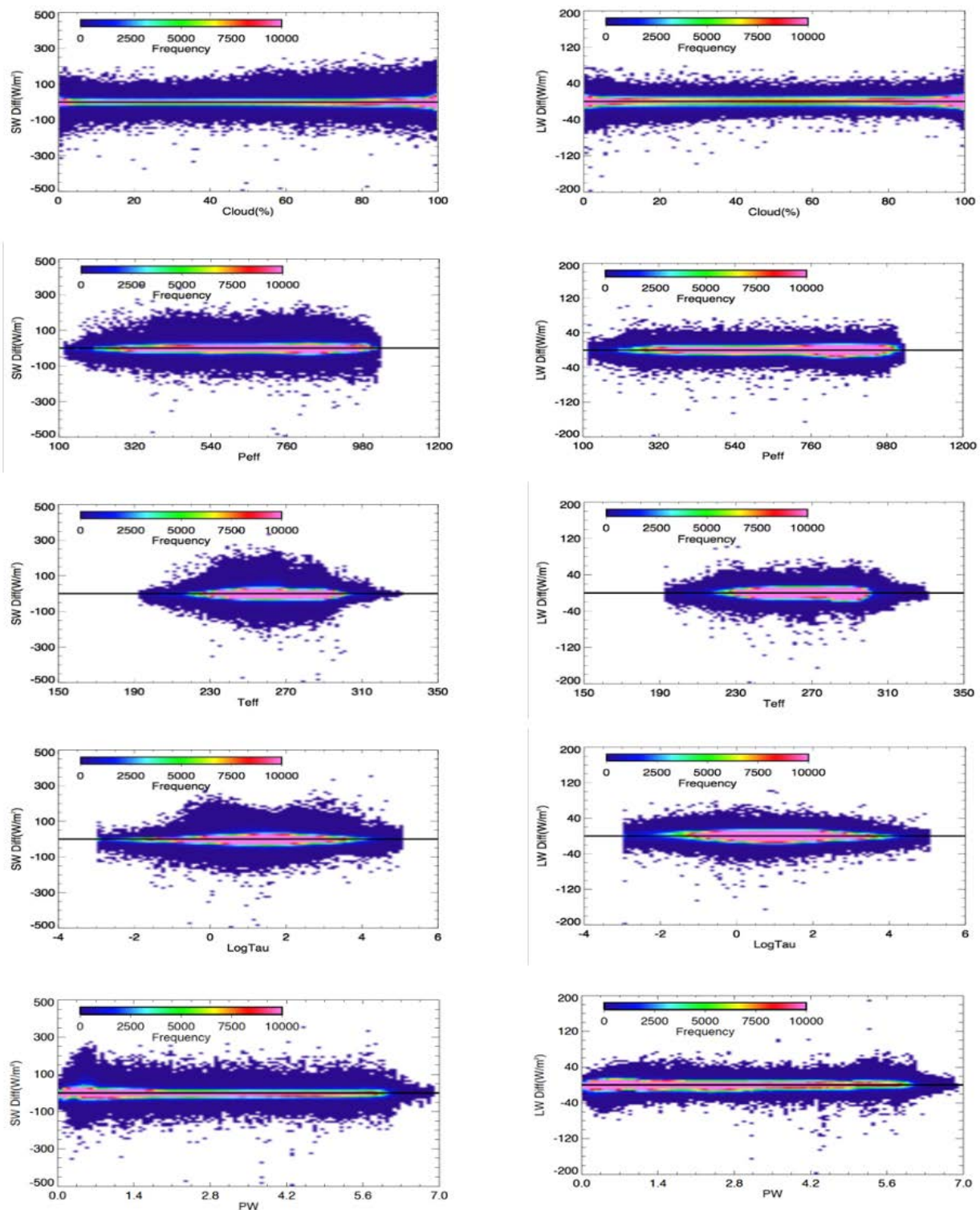
Figure 5-2. The FluxByCldTyp narrowband to broadband computed minus observed (left panels) SW and (right panel) LW non-homogeneous Terra and Aqua footprint flux ( \text{W m}^{-2} ) frequency plots during January 1-10, 2010 as a function of cloud fraction (%), cloud effective pressure (Peff in mb), cloud effective temperature (Teff in K), logarithm of cloud optical depth (LogTau), and precipitable water (PW in cm).
