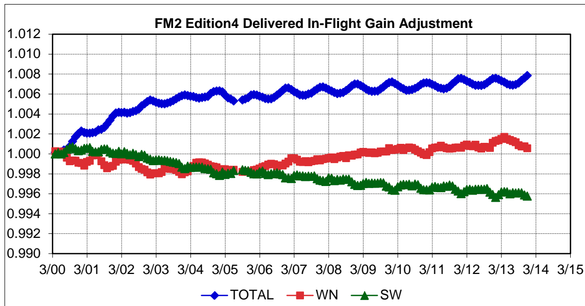
Figure 2-2 FM 2 Edition 4 In-Flight Gain Adjustment
