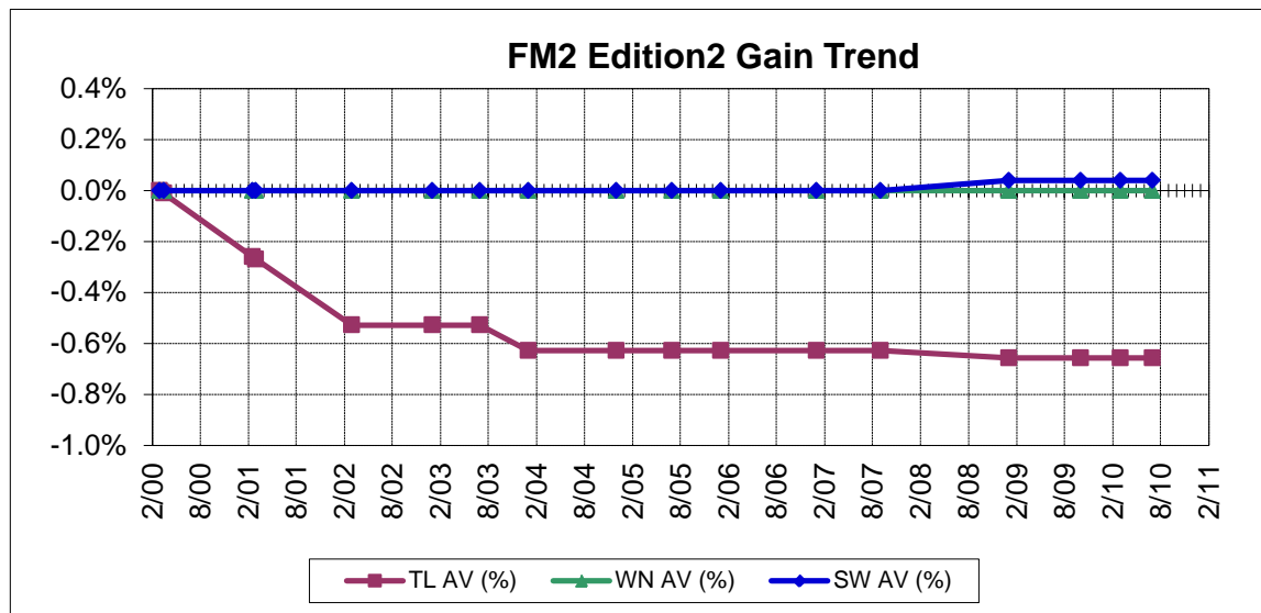
Figure 6-2 FM 2 Edition 2 In-Flight Gain Adjustment
