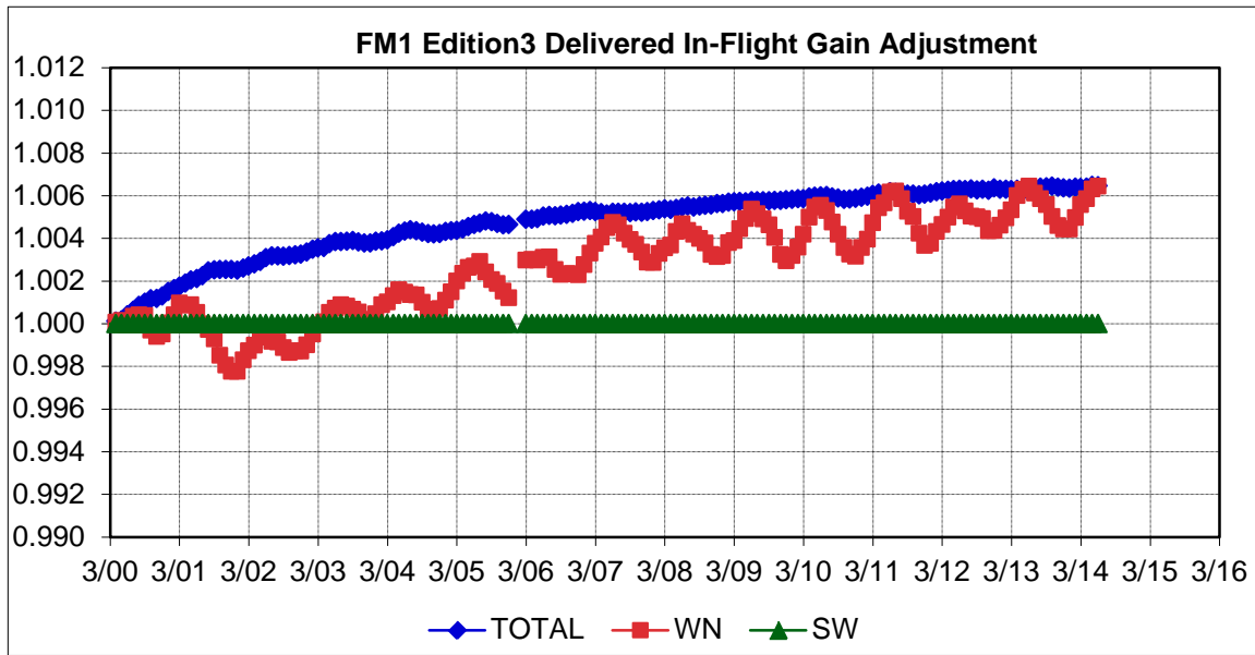
Figure 6-2 FM 1 Edition 3 In-Flight Gain Adjustment
