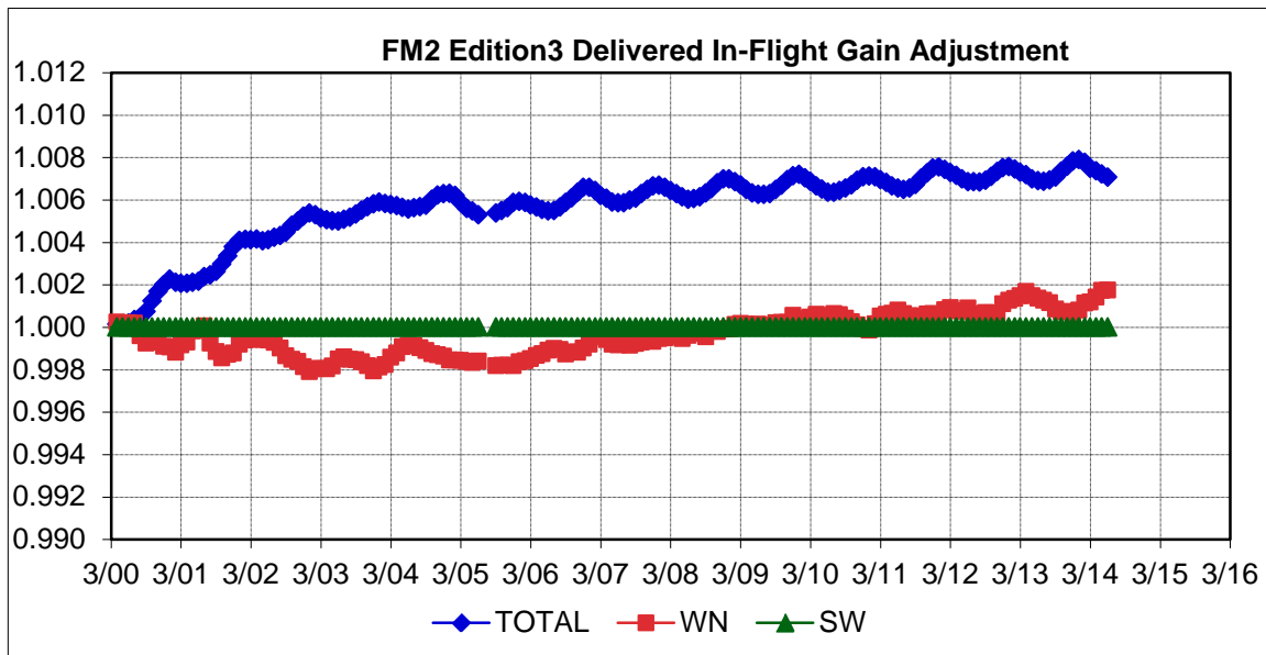
Figure 6-3 FM 2 Edition 3 In-Flight Gain Adjustment
