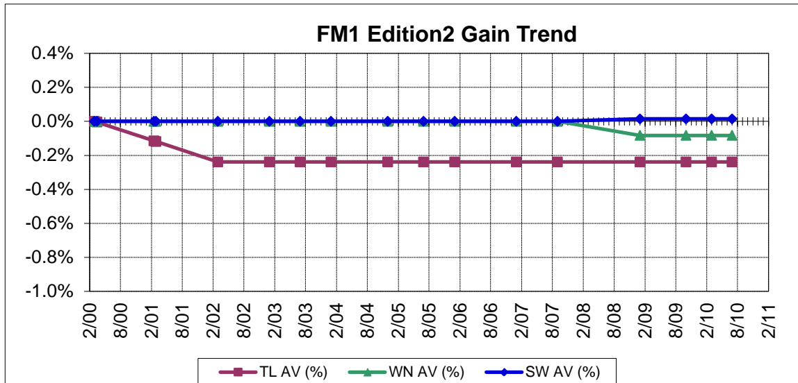
Figure 6-1 FM 1 Edition 2 In-Flight Gain Adjustment
