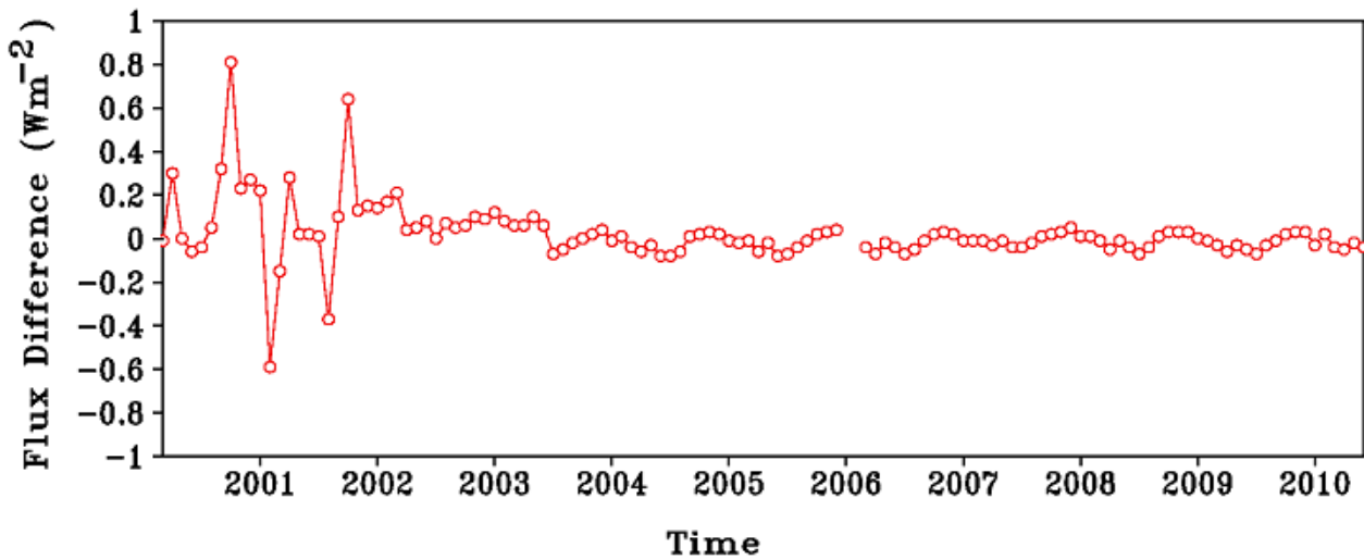
Figure 1. Time series of Terra Xtrk Edition3 minus FM1 Edition2_Rev1 global averaged monthly mean shortwave fluxes.
