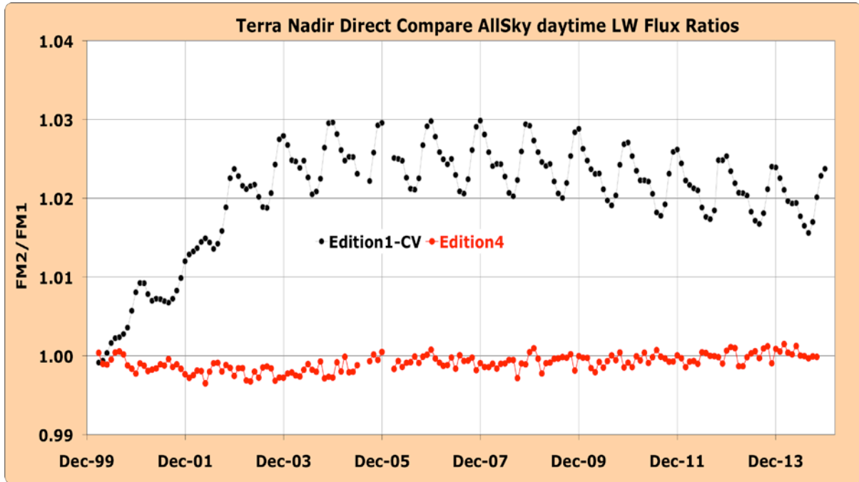
Figure 2-2. Terra nadir direct compare ratios for LW day time all sky fluxes.
