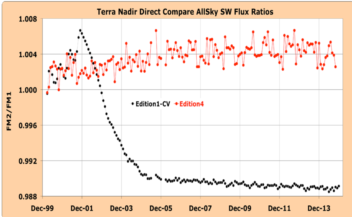
Figure 2-1. Terra nadir direct compare ratios for SW fluxes.
