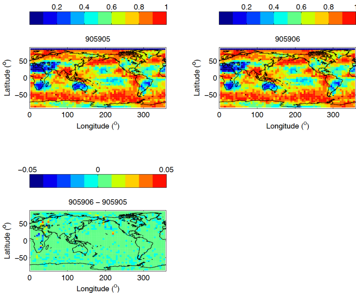
Figure 1. Monthly mean (Aug. 2008) cloud fraction derived over 5^{\circ} \times 5^{\circ} grid boxes from the 905905 version (top left) and from the 905906 version (top right). The difference is shown in the lower plot. The global monthly mean cloud fraction is 0.684 and 0.685 for 905905 and 905906, respectively.
