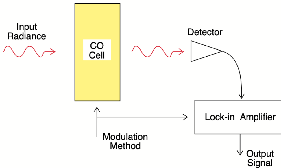
Figure 2.2.2 A basic correlation radiometry system.
