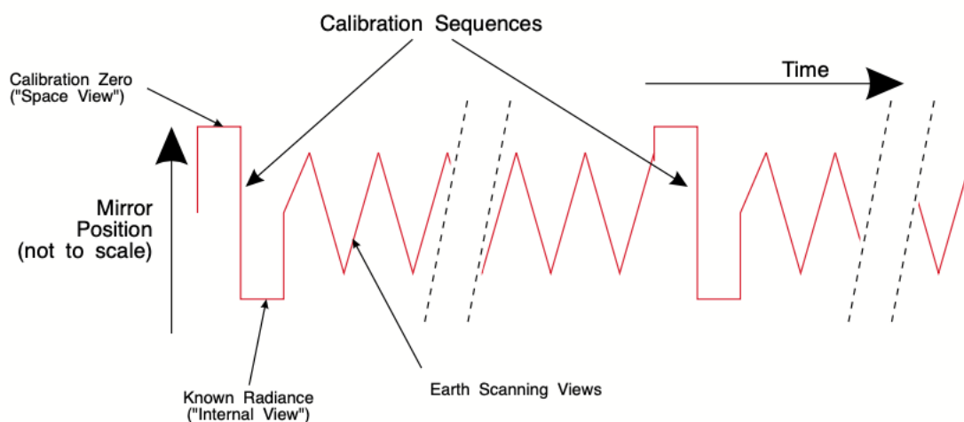
Figure 3.2.2 Typical MOPITT scanning sequence.
