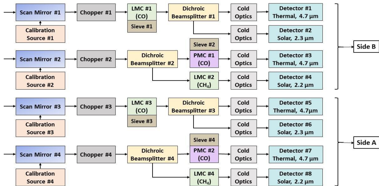
Figure 2.2.4 MOPITT optical channel diagram. Note that Side B is no longer functional due to the May 7 2001 cooler malfunction. Side A (Channels 5-8) continue to operate successfully. On August 2024, PMC #2 failed and remained off for the duration of the mission.
