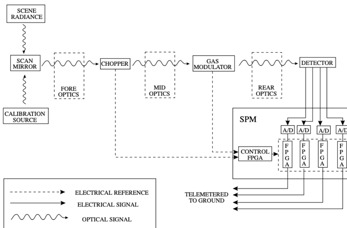
Figure 3.2.3 Single channel optical functional diagram.
