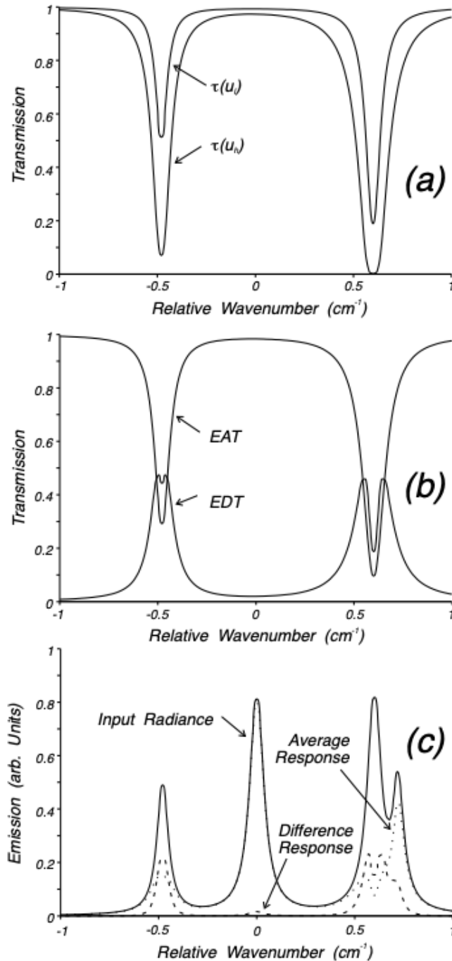
Figure 2.2.3 Operation of a correlation spectrometer in spectral space. EAT is the Equivalent Average Transmission. EDT is the Equivalent Difference
