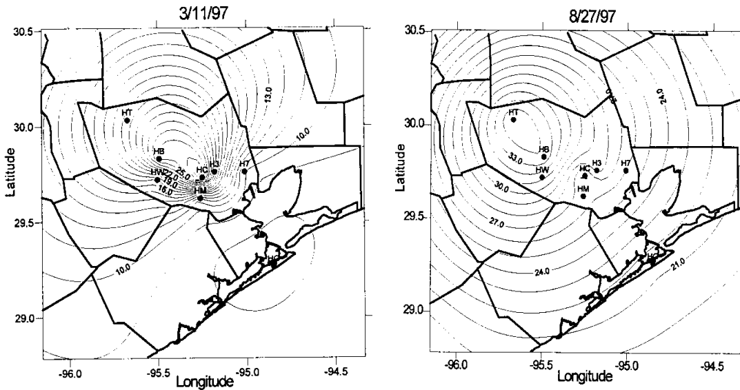
Figure 4.3.1-1. Concentrations of fine PM_{2.5} in the Houston area. The particulate matter isopleths shown in these plots were estimated (Lurmann, 1999) based on PM_{2.5} monitoring done at 8 locations in the Houston area (shown as dots in the Figure) between March 1997 and March 1998 (Tropp, et al., 1998). The data for 3/11/97 show high PM_{2.5} concentrations (isopleths are in \mu g/m^3 ) in the Ship Channel (industrial) area. The data for 8/27/97 show PM_{2.5} concentrations conditions when the peak concentrations are observed downwind of the urban core.
