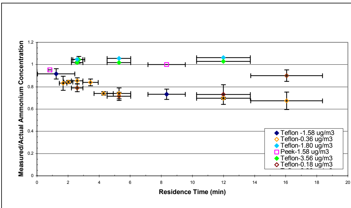
Figure 5. Residence time experiments run with Teflon and PEEK tubing. The legend indicates the concentrations of the ammonium solution injected into the ICs.
