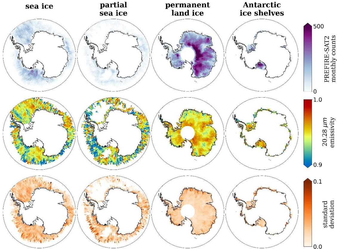
Figure 1-2: A sample of preliminary 3-SFC-SORTED-ALLSKY output for July 2024 showing PREFIRE-SAT2 channel 22 (20.28 \mu\text{m} ) gridded monthly counts (top), average surface emissivity (middle), and standard deviation of surface emissivity (bottom) for four Antarctic surface types. Data shown are for full granules and the average and standard deviation are taken with respect to the combination of all 8 cross-track scenes.
