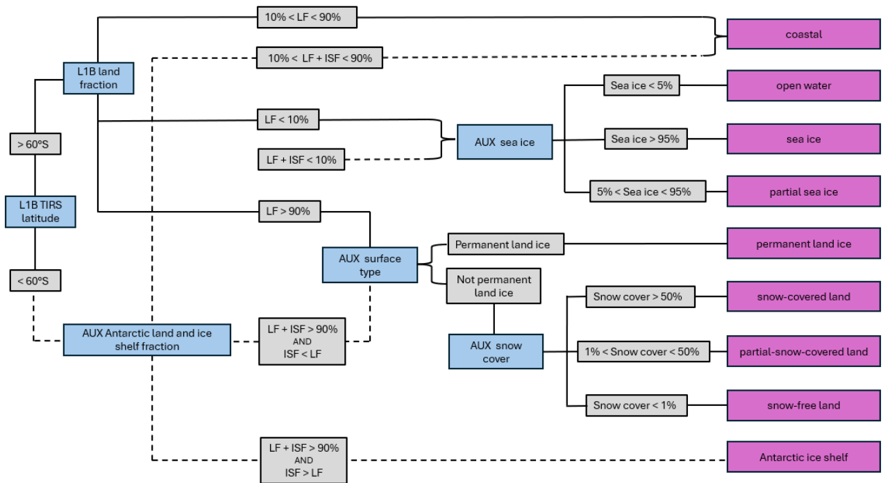
Figure 2-1: A flow chart summarizing the surface type designation used in the 3-SFC-SORTED-ALLSKY algorithm. LF and ISF denote land fraction and ice shelf fraction, respectively. AUX denotes PREFIRE Auxiliary data (AUX-SAT or, if unavailable, AUX-MET). The dashed lines represent the flow specific to observations at latitudes equal to or south of 60°S.
