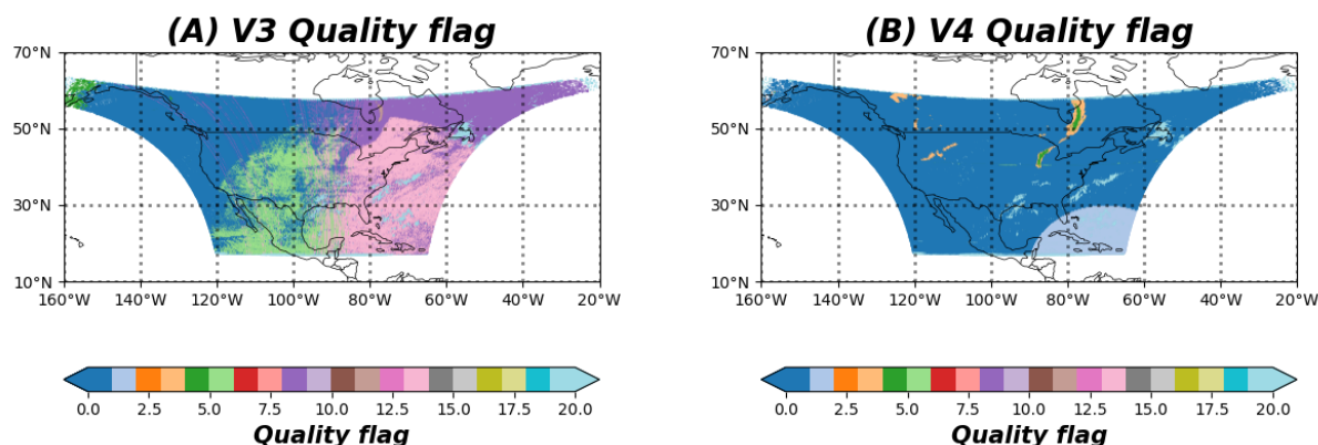
Figure 5. Comparison of the quality flag in the TEMPO O3TOT product for the same scan: V03 (left) and V04 (right).
