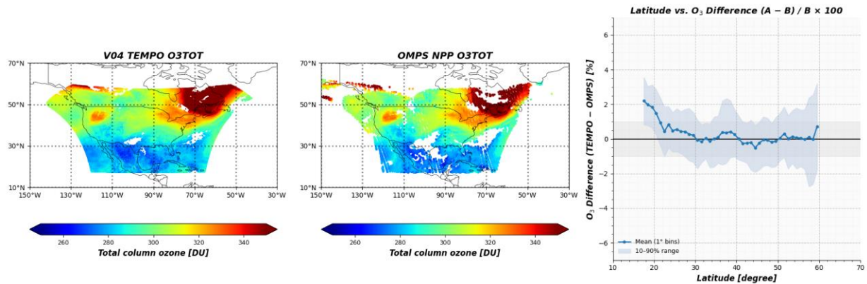
Figure 3. Comparison between total column ozone from the V04 TEMPO O3TOT product and the OMPS NPP O3TOT product. (left) Spatial distribution of the total column ozone from the V04 TEMPO O3TOT product on September 03, 2024 (S008). (middle) Spatial distribution of the total column ozone from the OMPS NPP product on September 03, 2024 (S008). (right) Relative difference between TEMPO and OMPS NPP as a function of wavelength.
