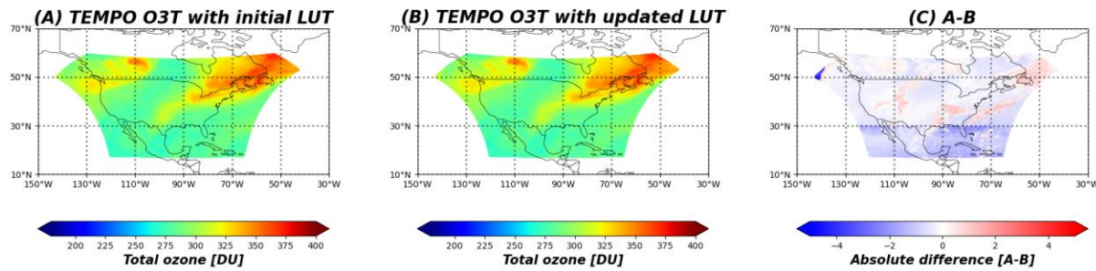
Figure 1. Effect of the Look-Up Table (LUT) updates on total column ozone retrieval on July 26, 2025. (left) Retrieval using the updated V04 TEMPO O3TOT algorithm with the initial LUT used in the V03 TEMPO O3TOT algorithm. (middle) Retrieved using the updated V04 TEMPO O3TOT algorithm with the updated LUT used in the V04 TEMPO O3TOT algorithm. (right) Absolute difference between (A) and (B).
