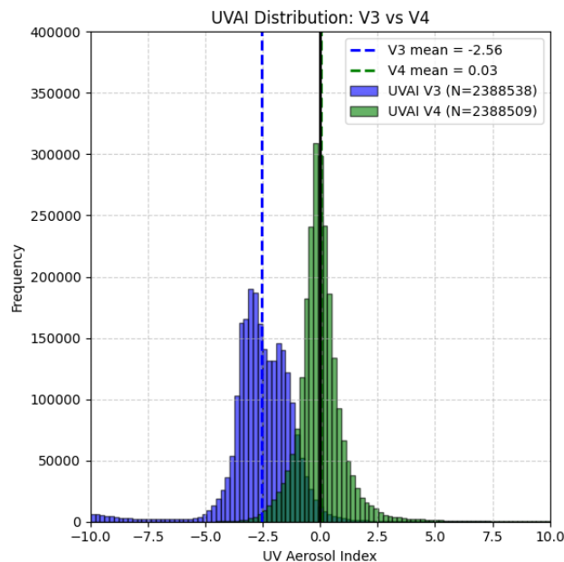
Figure 4. Comparison of the UVAI in the TEMPO O3TOT product for the same scan on September 3, 2024. Blue and green bars represent the UVAI from V03 TEMPO O3TOT and V04 TEMPO O3TOT, respectively. Blue and green dashed lines represent the mean value of each UVAI.
