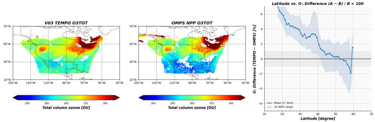
Figure 2. Comparison between total column ozone from the V03 TEMPO O3TOT product and the OMPS NPP O3TOT product. (left) Spatial distribution of the total column ozone from the V03 TEMPO O3TOT product on September 03, 2024 (S008). (middle) Spatial distribution of the total column ozone from the OMPS NPP product on September 03, 2024 (S008). (right) Relative difference between TEMPO and OMPS NPP as a function of wavelength.
