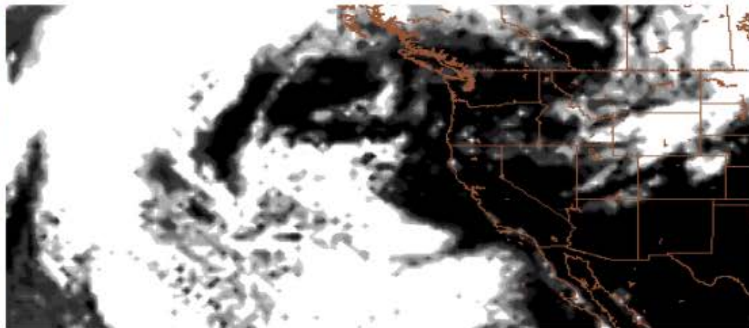
Total Clouds
