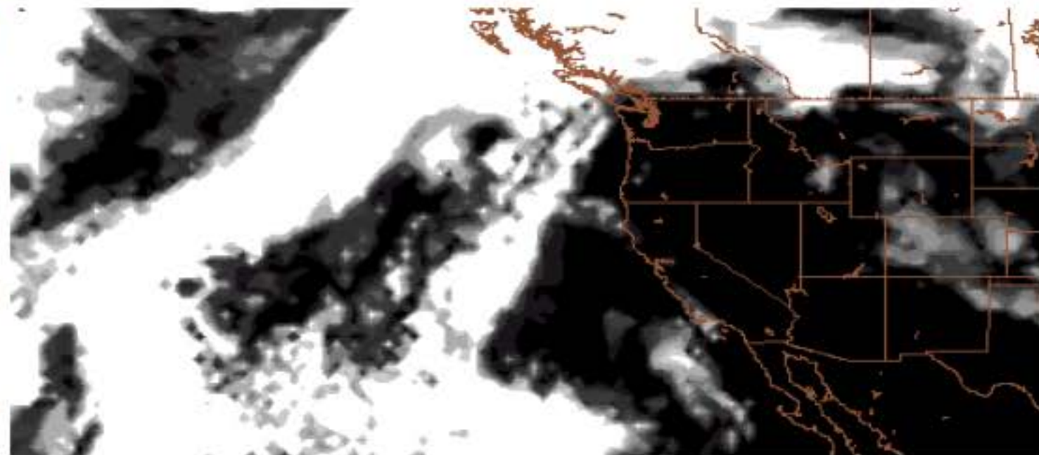
Total Clouds
