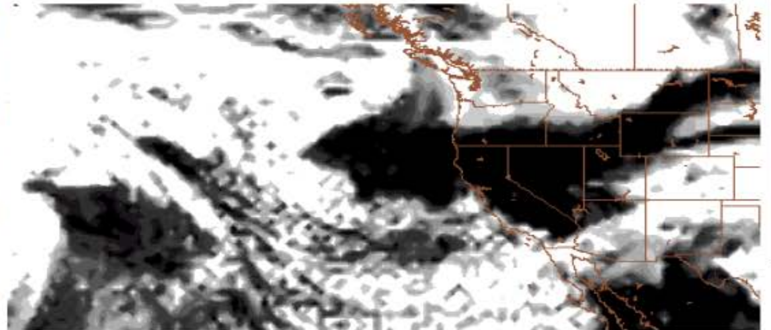
Total Clouds
