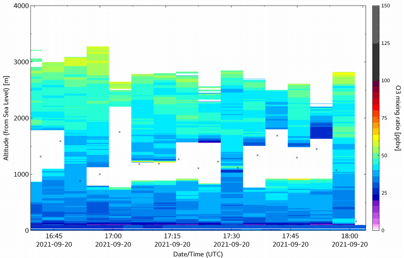
LMOL University of Houston 2021-09-20 - Tracer AQ - Level 2
