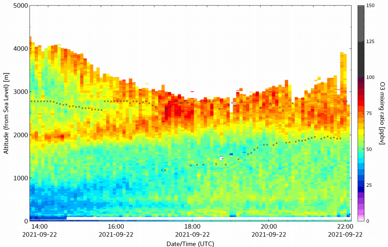
LMOL University of Houston 2021-09-22 - Tracer AQ - Level 2
