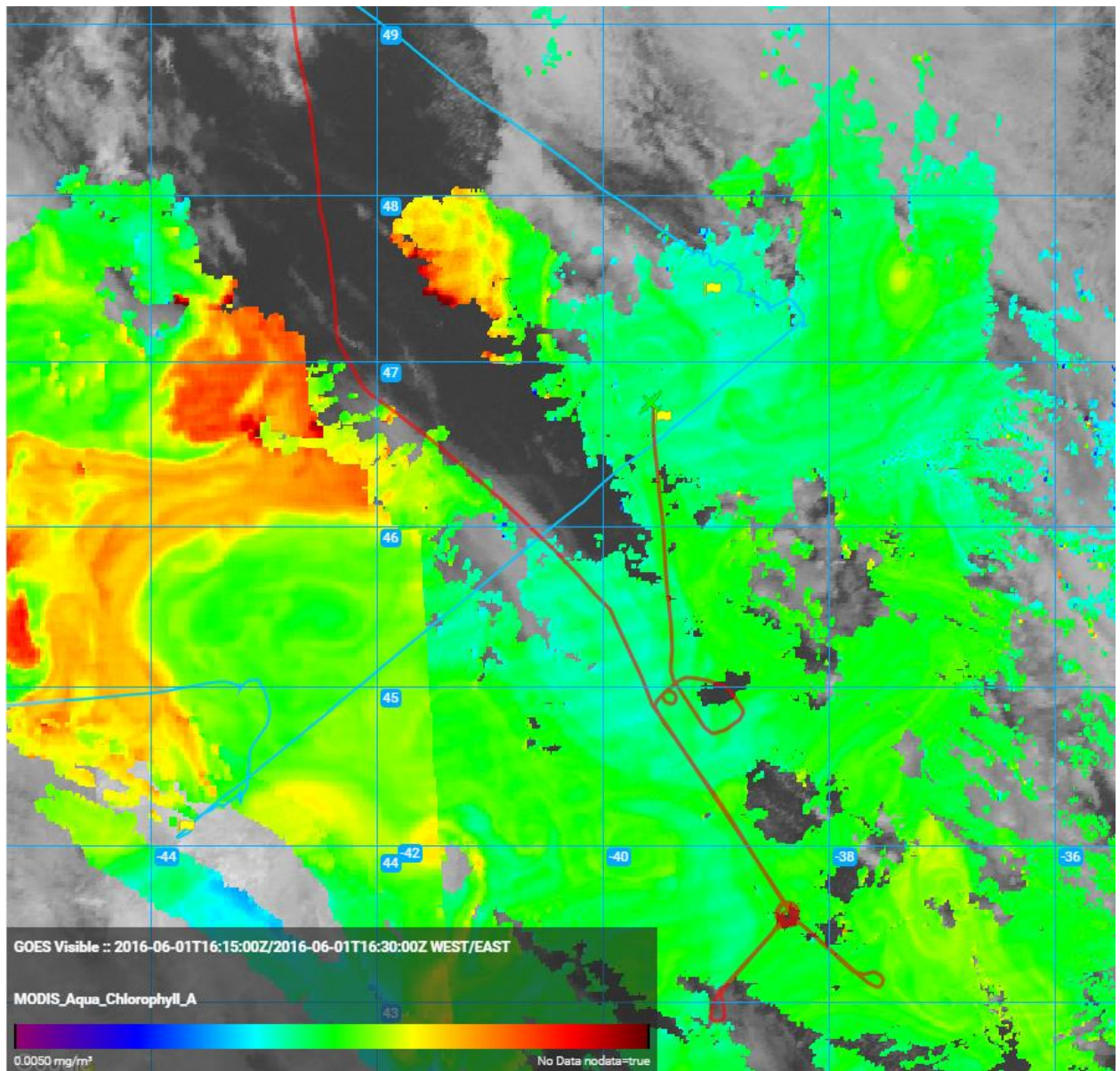
1640Z_FloatOverflightWithMay24thChlorophyll
