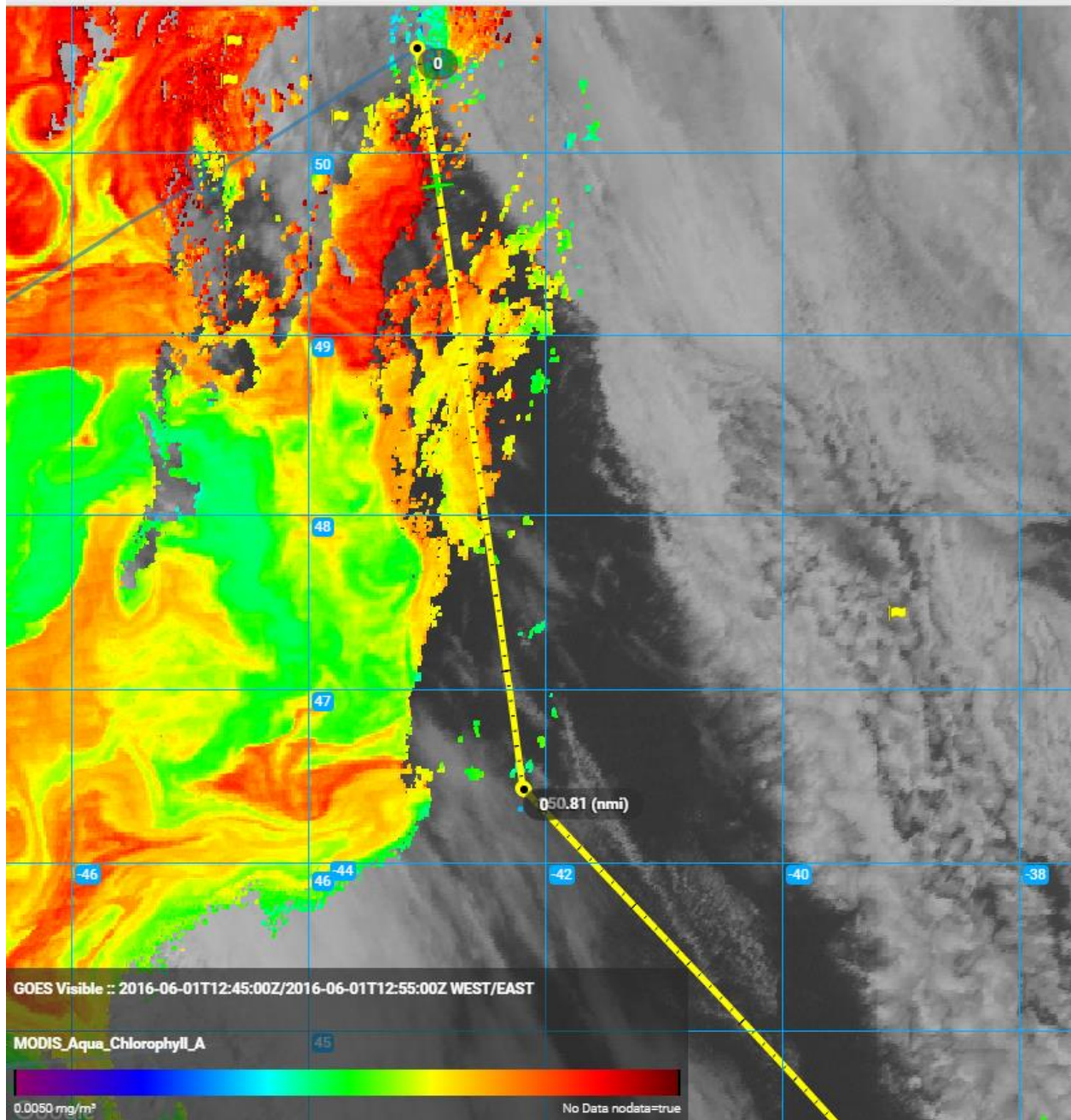
1310Z_SouthboundHighAltRunWithMay30thChlorophyll
