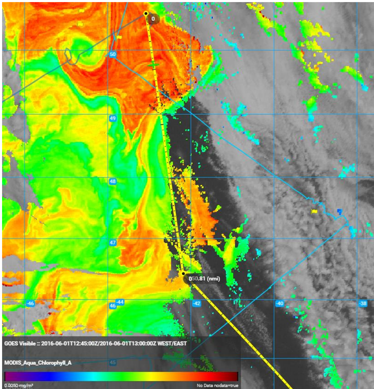
1310Z_SouthboundHighAltRunWithMay23rdChlorophyll
