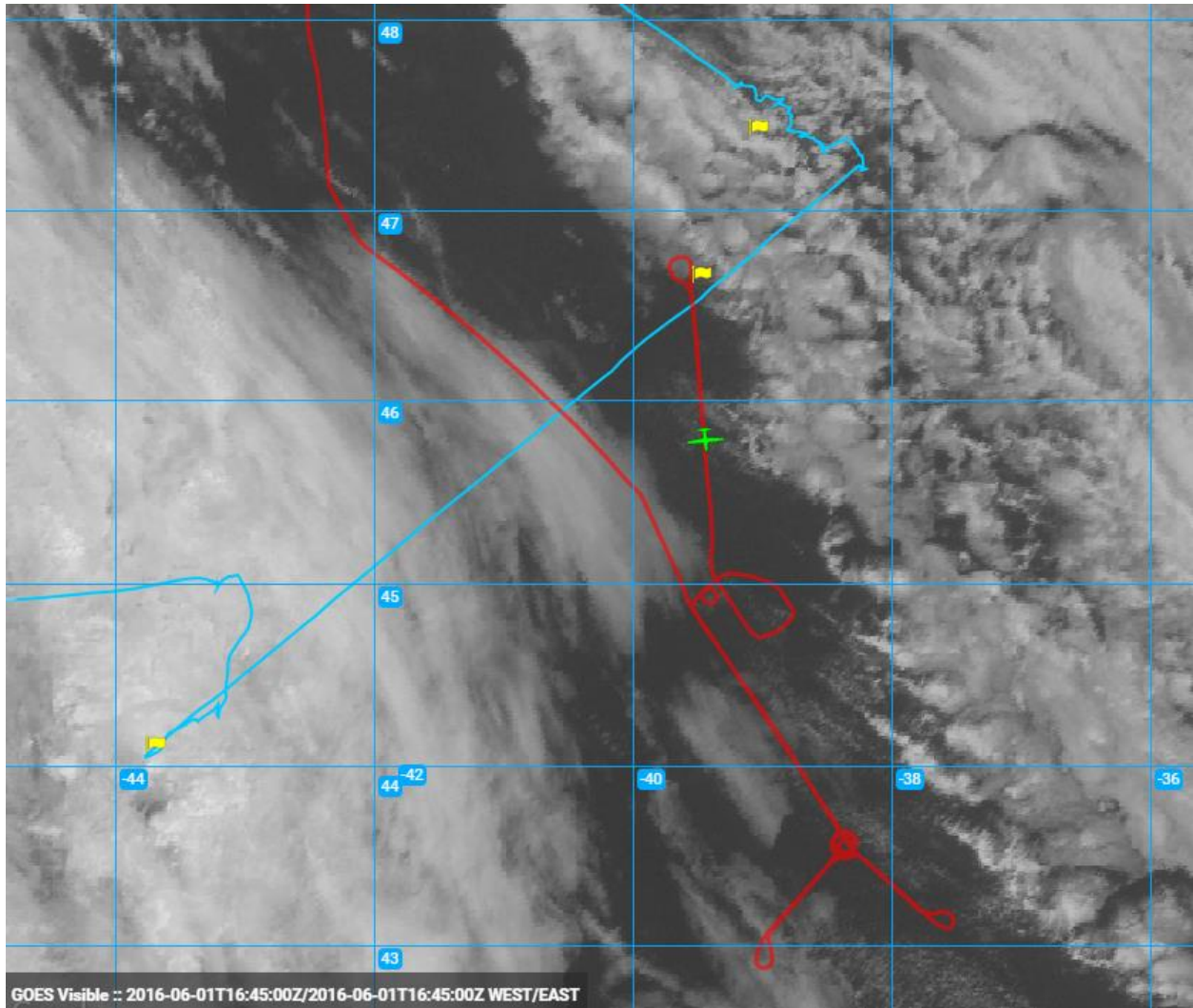
1700Z_InlineDescentBackDownFromFloatOverflight
