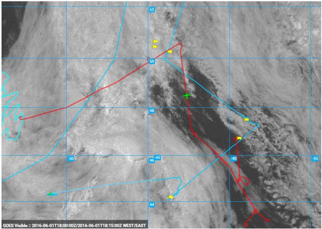
1830Z_LowLevelLeg
