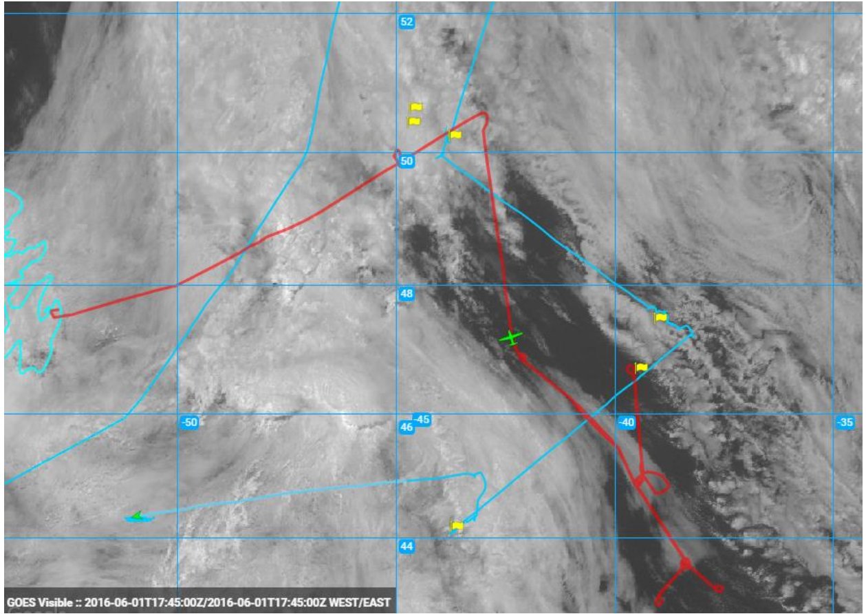
1810Z_LowLevelLeg
