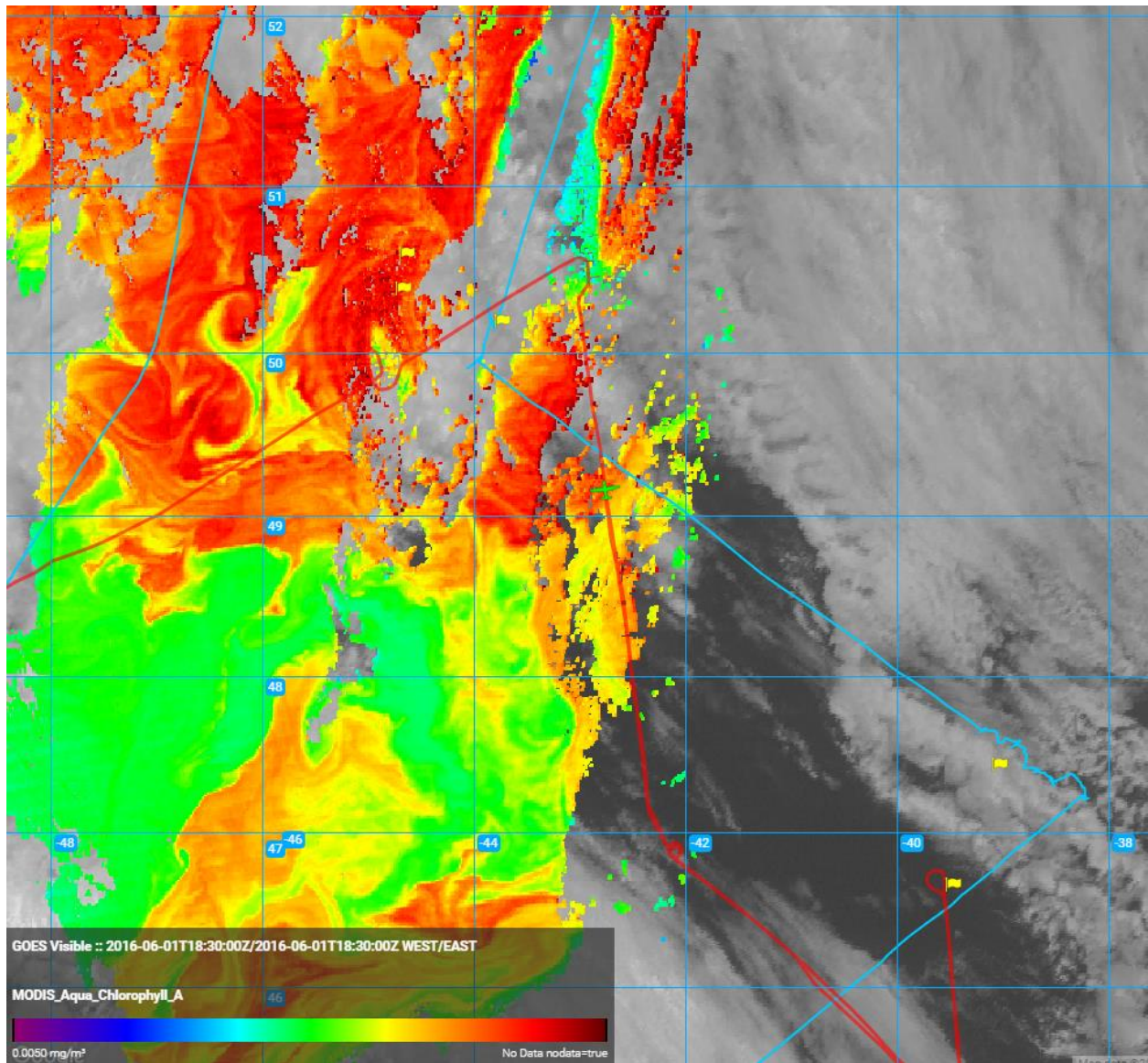
1850Z_LowLevelLegIntoTheBloomAroundS3
