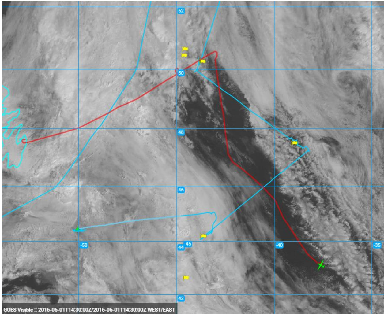
1440Z_SouthernPointOfHighAltSurvey_ZoomedOut
