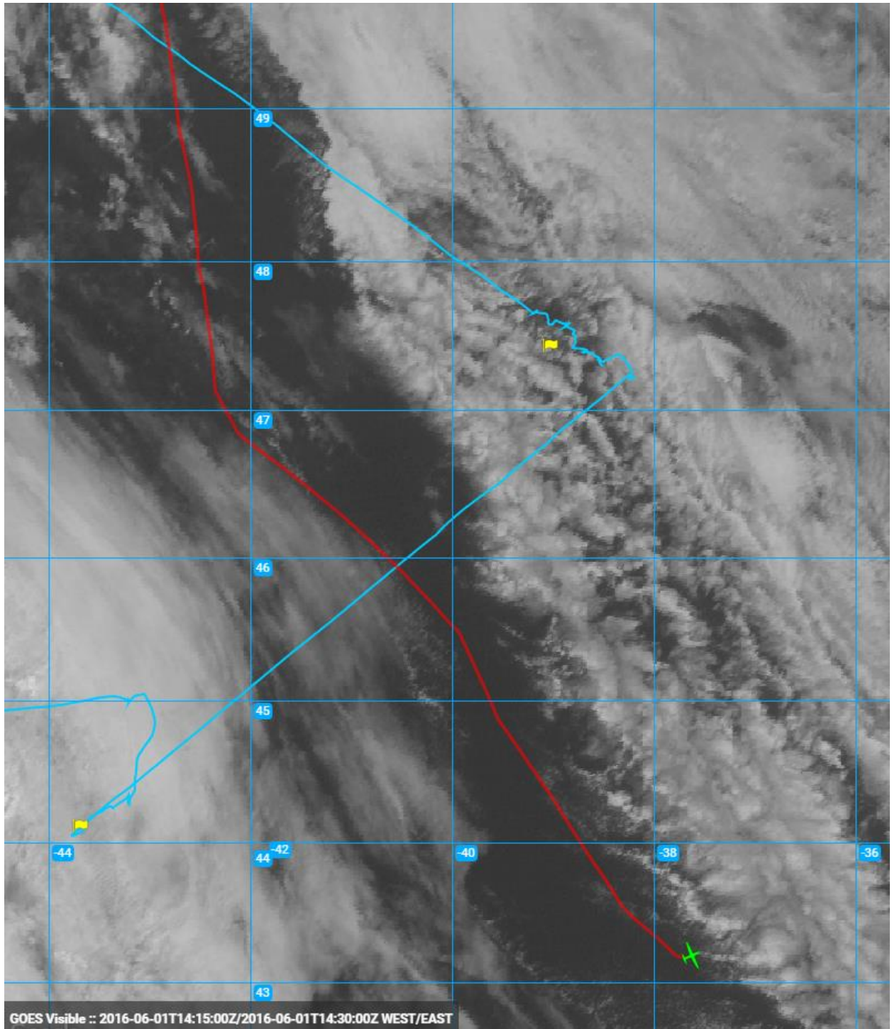
1440Z_SouthernPointOfHighAltSurvey
