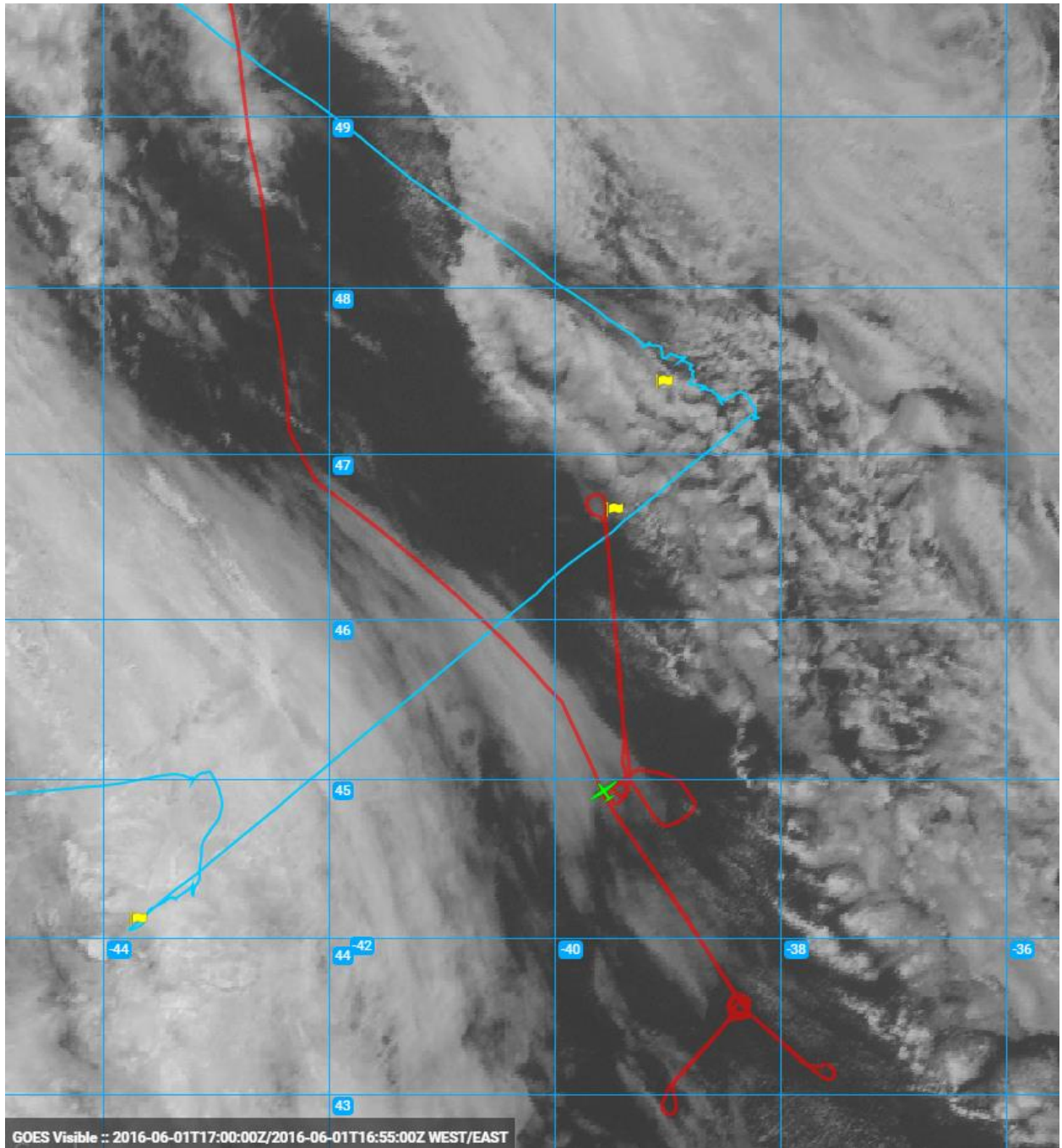
1710Z_LowLevelBackToTheNorth
