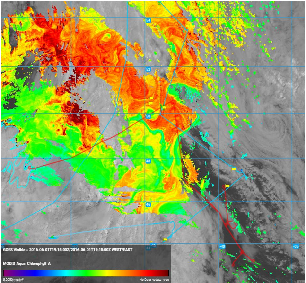
1930Z_RTbwithMay23rdChlorophyll
