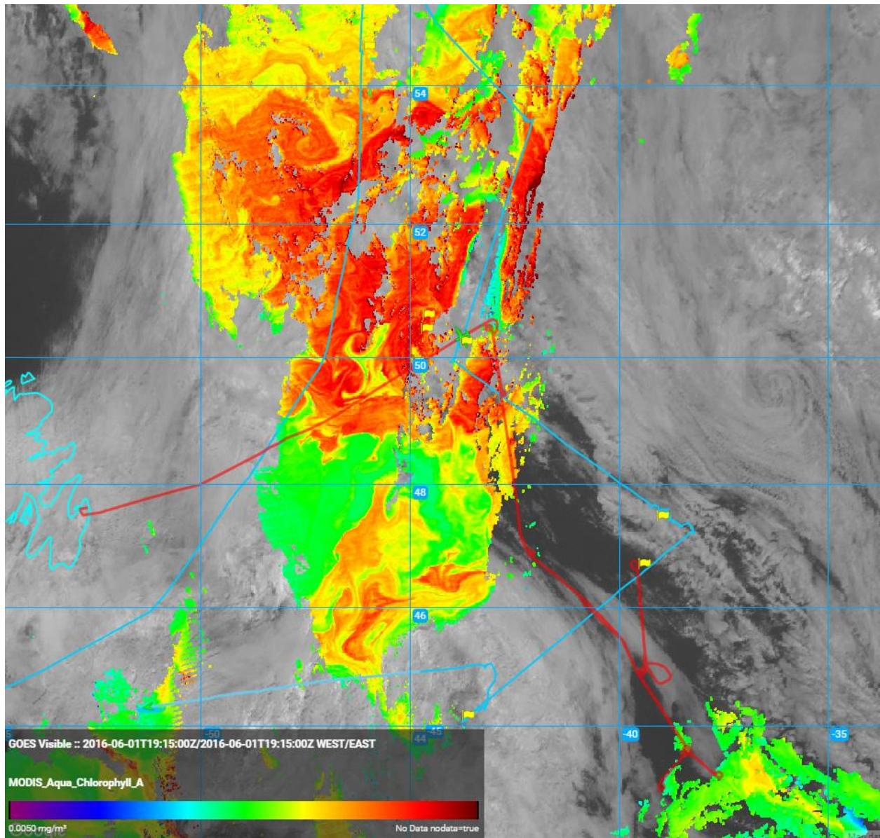
1930Z_RTbwithMay30thChlorophyll
