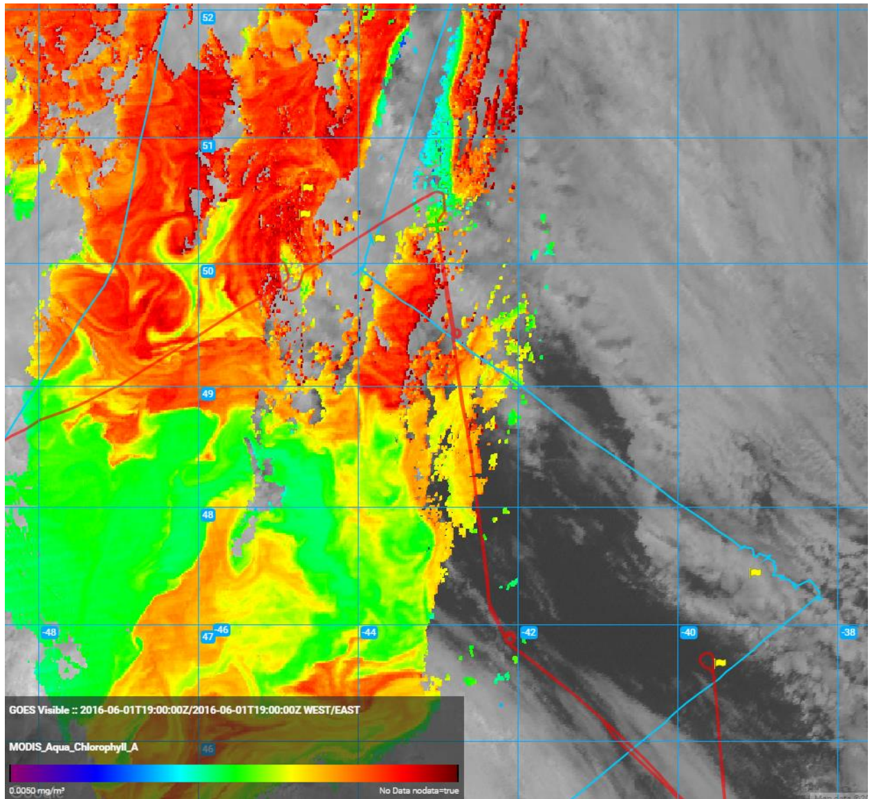
1915Z_LowLevelLegIntoTheBloomAroundS3
