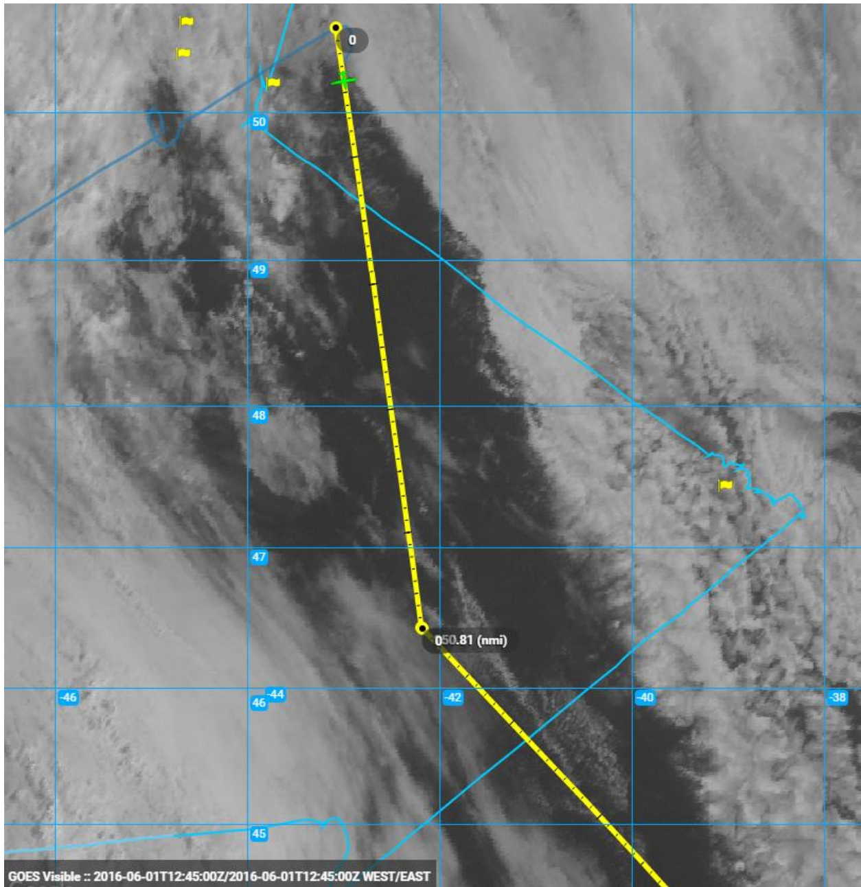
1300Z_SouthboundHighAltRun
