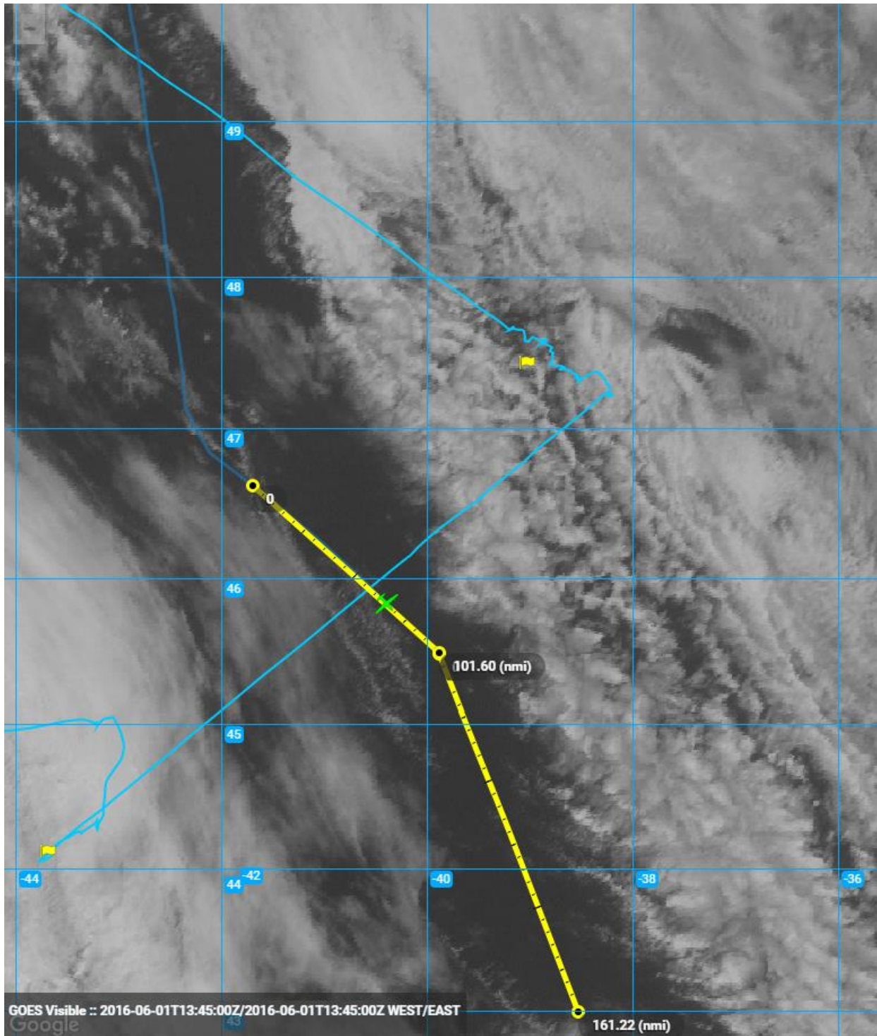
1400Z_SouthboundHighAltRunOnTheKink
