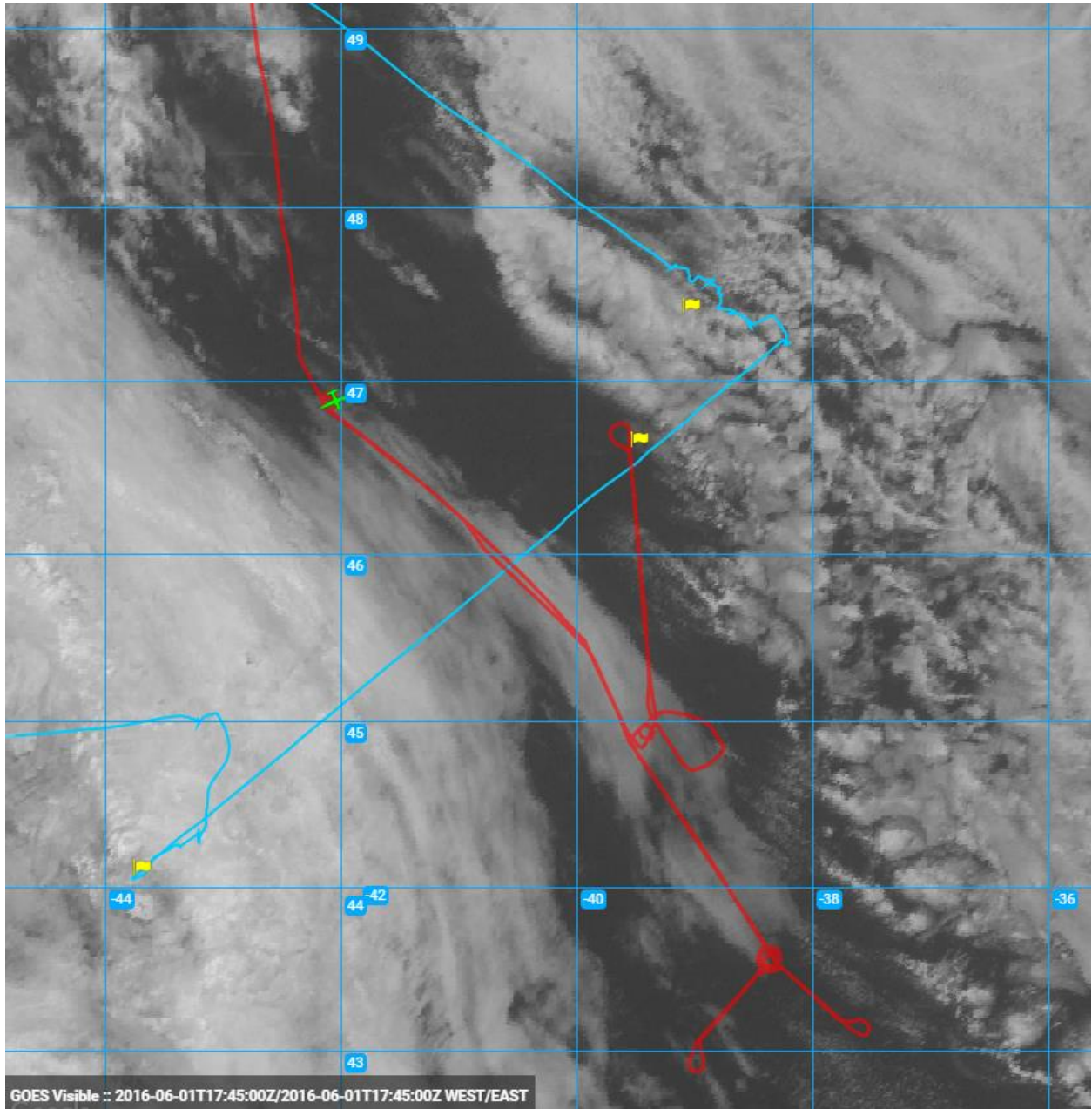
1800Z_ShortSpiral
